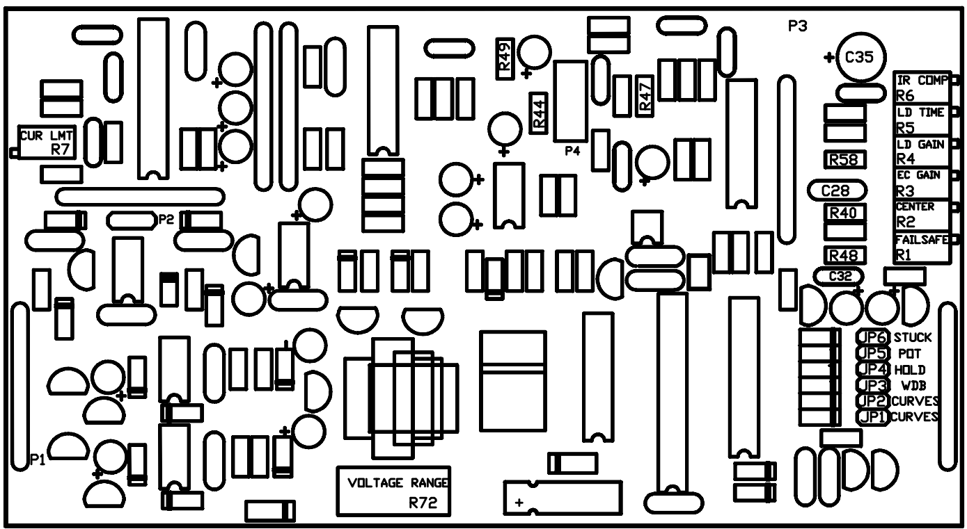
WIRING DIAGRAM
